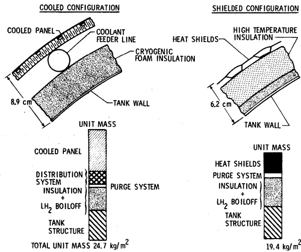
Figure 21. Comparison of convectively cooled and shielded tank structures.
