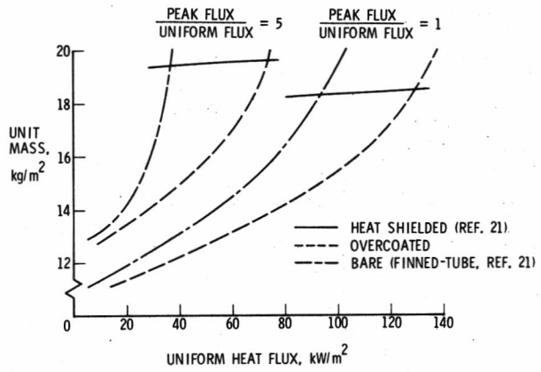
Figure 16. Convectively cooled panel masses.
