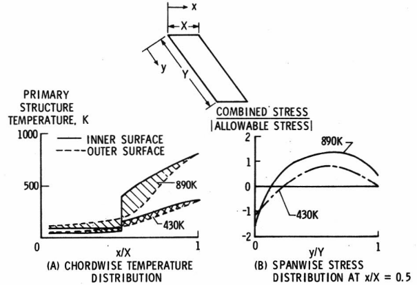
Figure 11. Strut temperature and stress distributions for coolant outlet temperatures of 430 K and 890 K.
