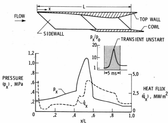
Figure 3. Typical design loads - sidewall.
