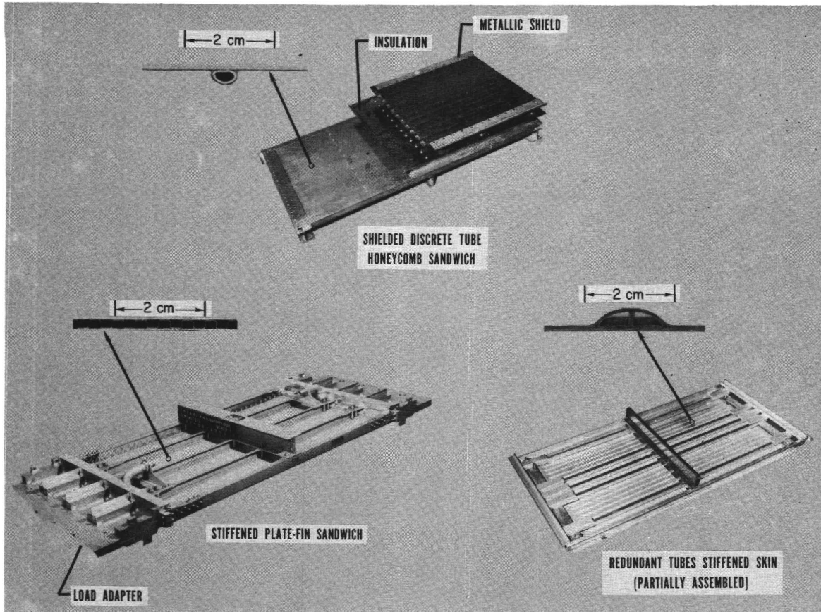
Figure 22. Large (0.61 by 1.22 m) convectively cooled test panels with cooling passage details.
