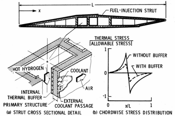
Figure 10. Internal thermal-buffer concept.
