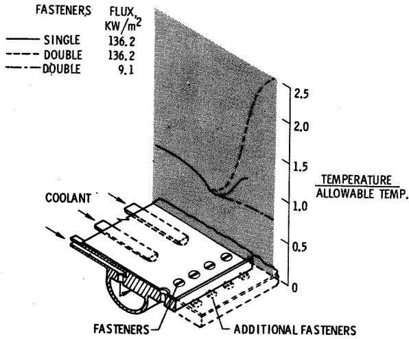
Figure 19. Effect of absorbed heat flux on joint design.
