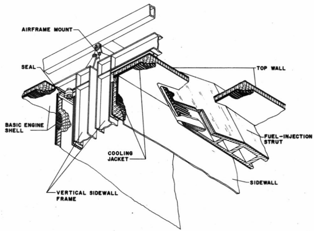
Figure 4. Typical construction of engine shell and fuel-injection strut.
