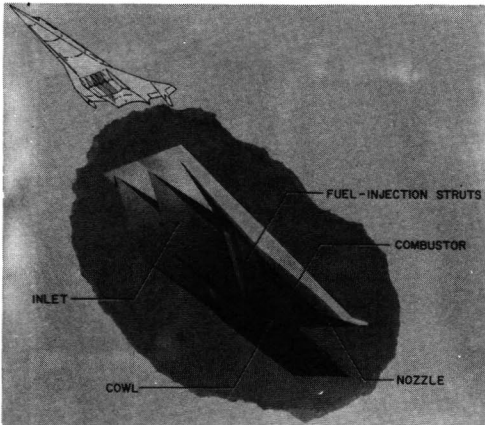
Figure 2. Airframe-integrated supersonic combustion ramjet.
