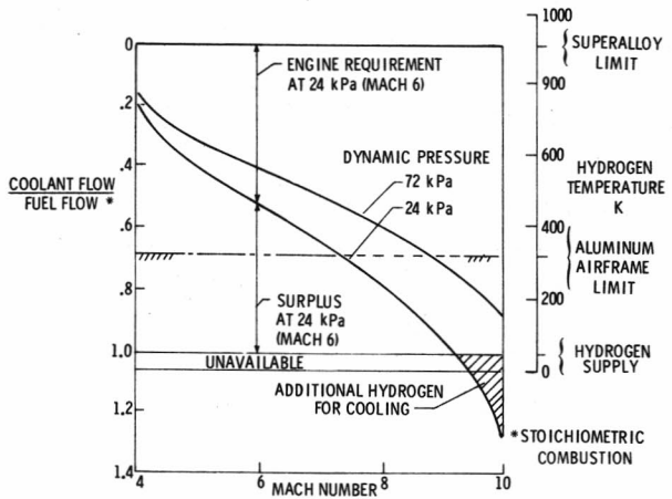
Figure 13. Engine cooling requirements.
