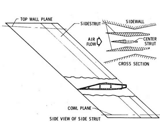
Figure 8. Fuel-injection struts.
