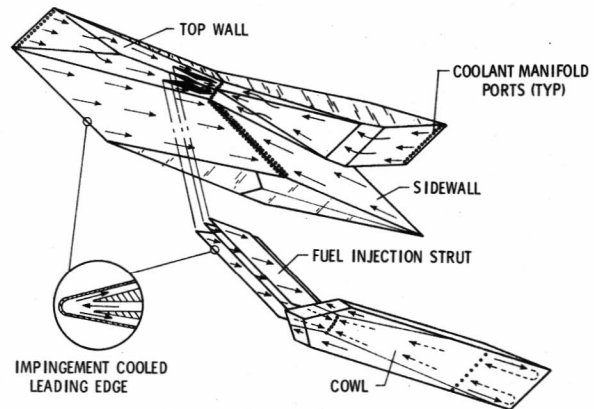
Figure 5. Hydrogen coolant routing scheme (One sidewall removed).
