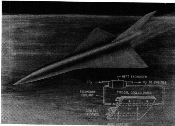
Figure 14. Convective cooling system for hypersonic aircraft.
