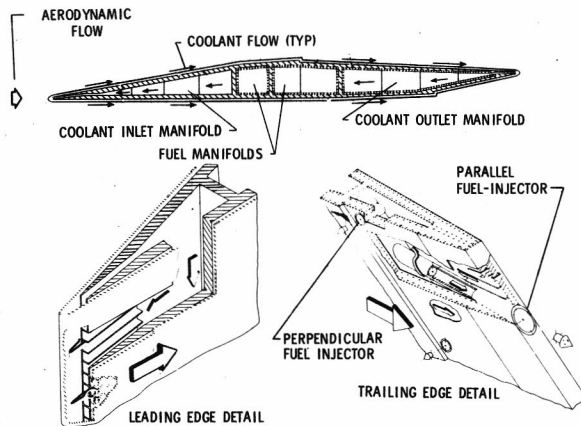
Figure 9. Fuel-injection strut detail.
