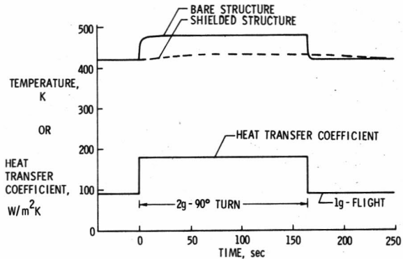
Figure 17. Sensitivity of convectively cooled structures to transient heat loads.
