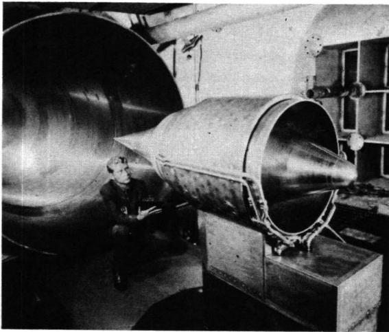
Figure 1. Hypersonic Research Engine (rear view) installed in the Langley 8-Foot High Temperature Structures Tunnel.
