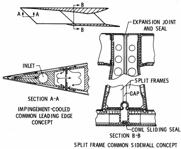
Figure 7. Leading edge and sidewall concept.
