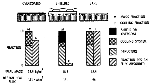
Figure 20. Mass and cooling characteristics of convectively cooled structures.
