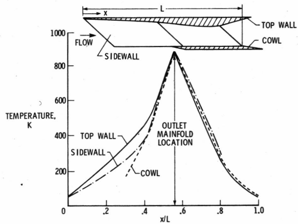
Figure 6. Engine component temperature distributions.
