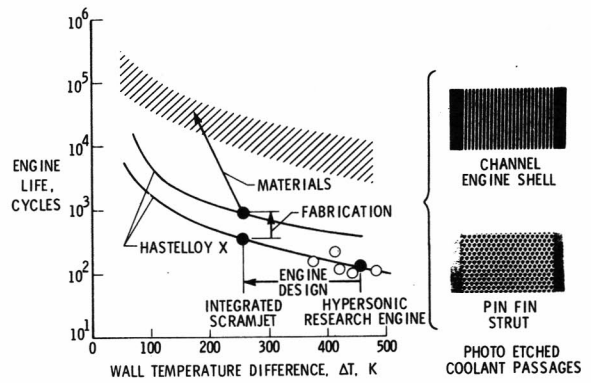
Figure 12. Factors improving thermal fatigue life.
