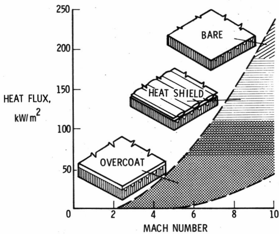
Figure 15. Recommended application regions for convectively cooled airframe structures.
