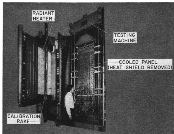
Figure 23. Test apparatus for convectively cooled structures.
