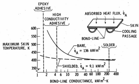
Figure 18. Effect of bond-line conductance on maximum skin temperature for bare and shielded configurations.
